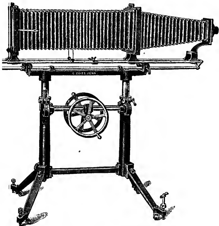
FIG. 67.—Photo-micrographic camera.
